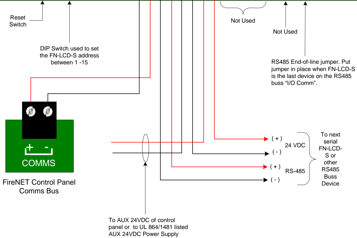
FN-LCD-S Wiring Detail
